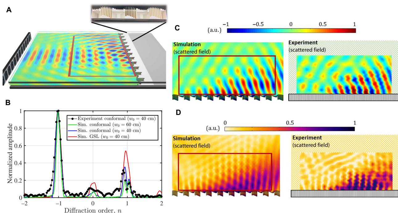
Fig. 3. Experimental verification. (A) Schematic representation of the experimental setup and a photograph of the fabricated sample. (B) Comparison between the normalized scattering of the anomalous reflective metamirrors for different beam widths, w_0 : simulation (sim.) of the conformal metamirror ( w_0 = 40 and 60 cm), experimental verification of the conformal metamirror ( w_0 = 40 cm), and simulated GSL design ( w_0 = 40 cm). The normalized scattering is calculated with a Fourier transform of the pressure fields along a line over the metasurfaces. (C and D) Analysis of the real part (C) and the magnitude square (D) of the experimental pressure field and the comparison with numerical simulations. a.u., arbitrary units.
